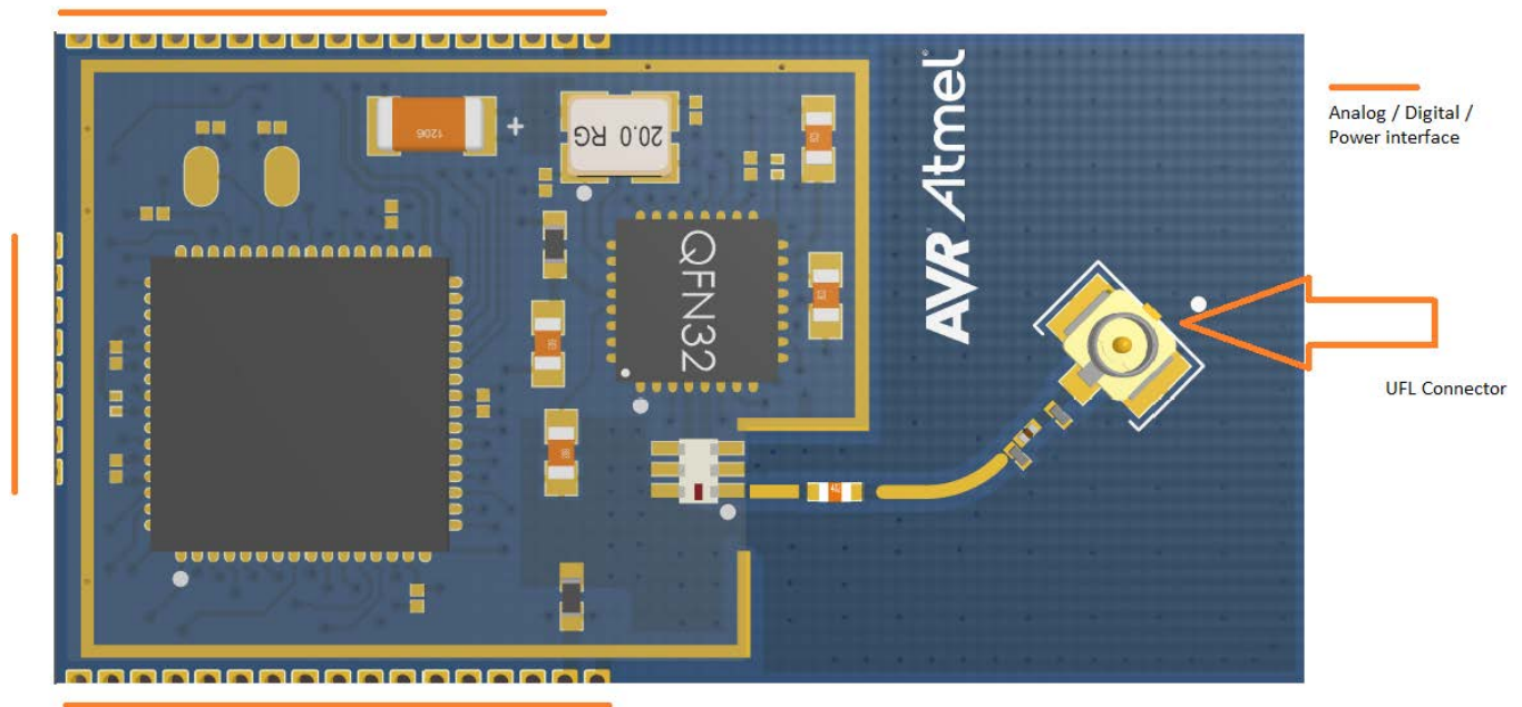
Figure 2-1. ATZB-X0-256-4-0-U User Interface Diagram
