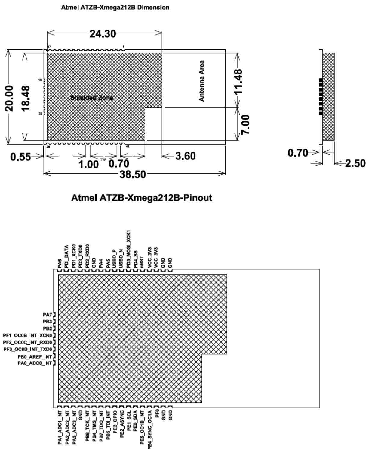
Figure 3-1. ATZB-X0-256-4-0-U Dimensions and Pinout
